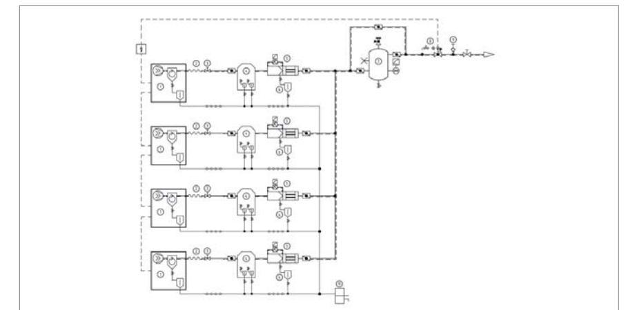
Fig. 2c: P+I diagram of a compressed air station
