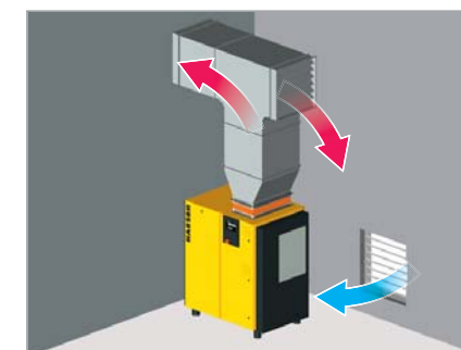
Fig. 4: A thermostatically-controlled flap directs warm air into the compressor room in winter
