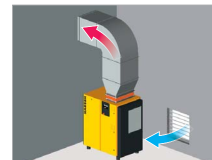
Fig. 3: Forced ventilation with exhaust ducting for machines above 11 kW
