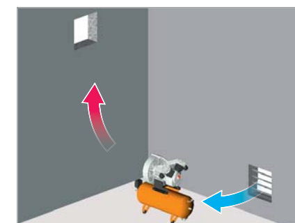
Fig. 1: Natural ventilation for compressors up to 5.5 kW
